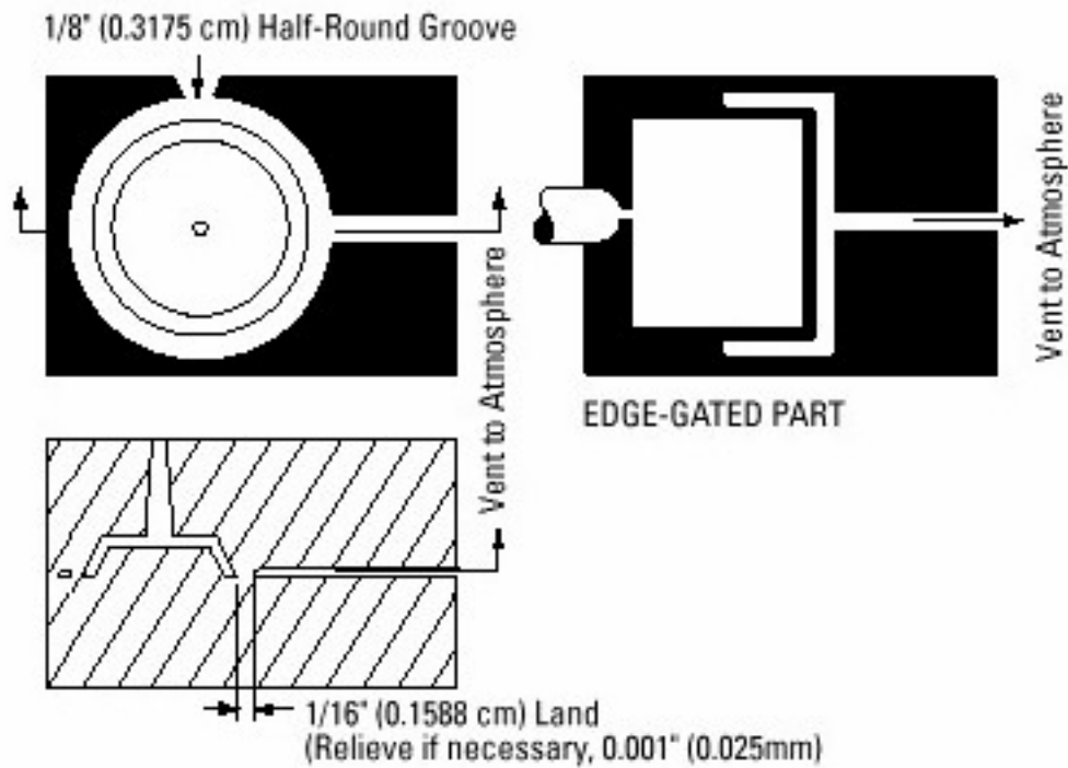
Figure3-7. Continuous Venting Techniques.
