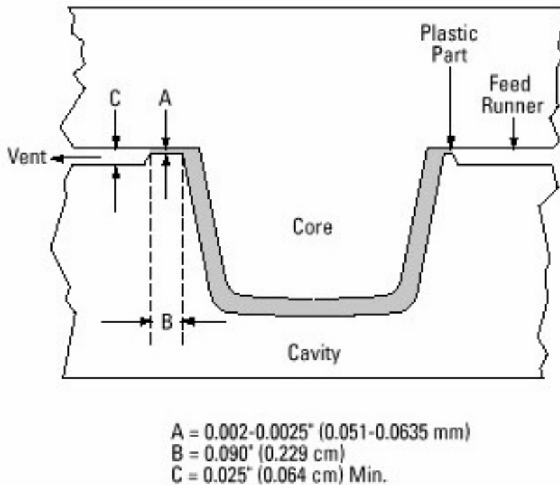
Figure 3-6. Conventional Parting Line vent.
