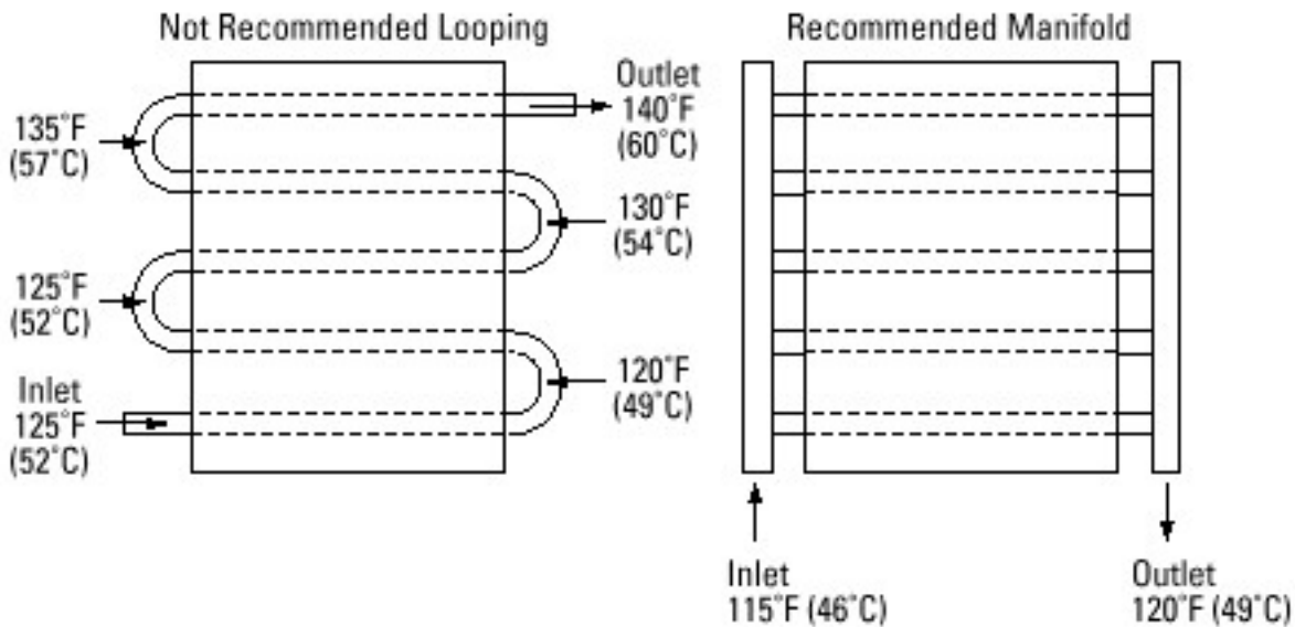
Figure 3-9. Cooling Channels
