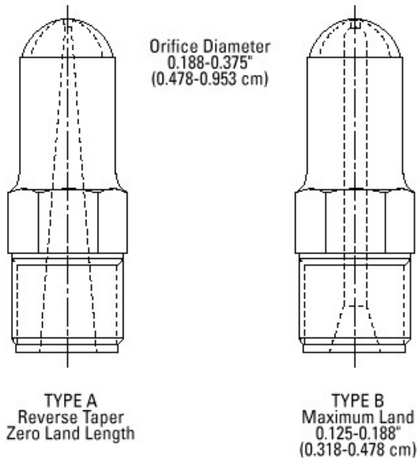
Figure 3-11. Nozzle Designs.
