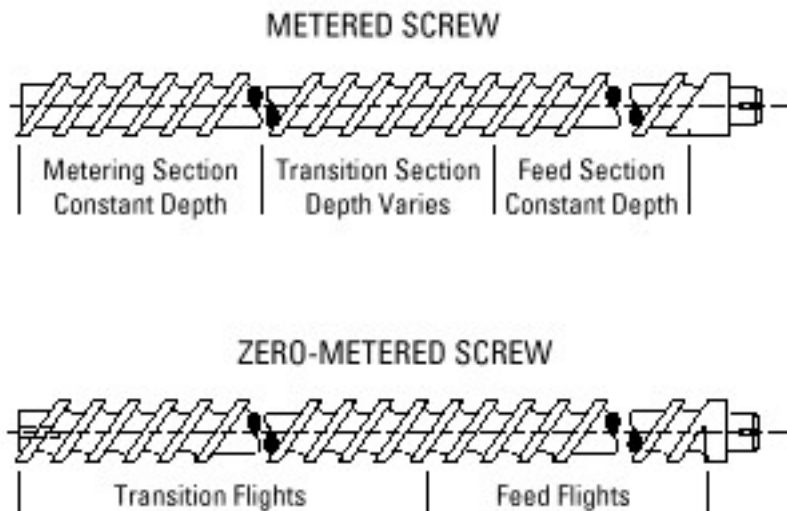
Figure 3-10. Screw Designs.
