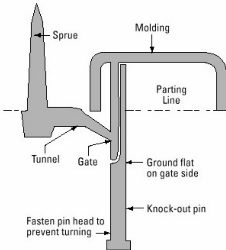
Figure 3-4. Tunnel Gating
