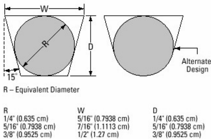
Figure 3-1. Trapezoidal Runners
