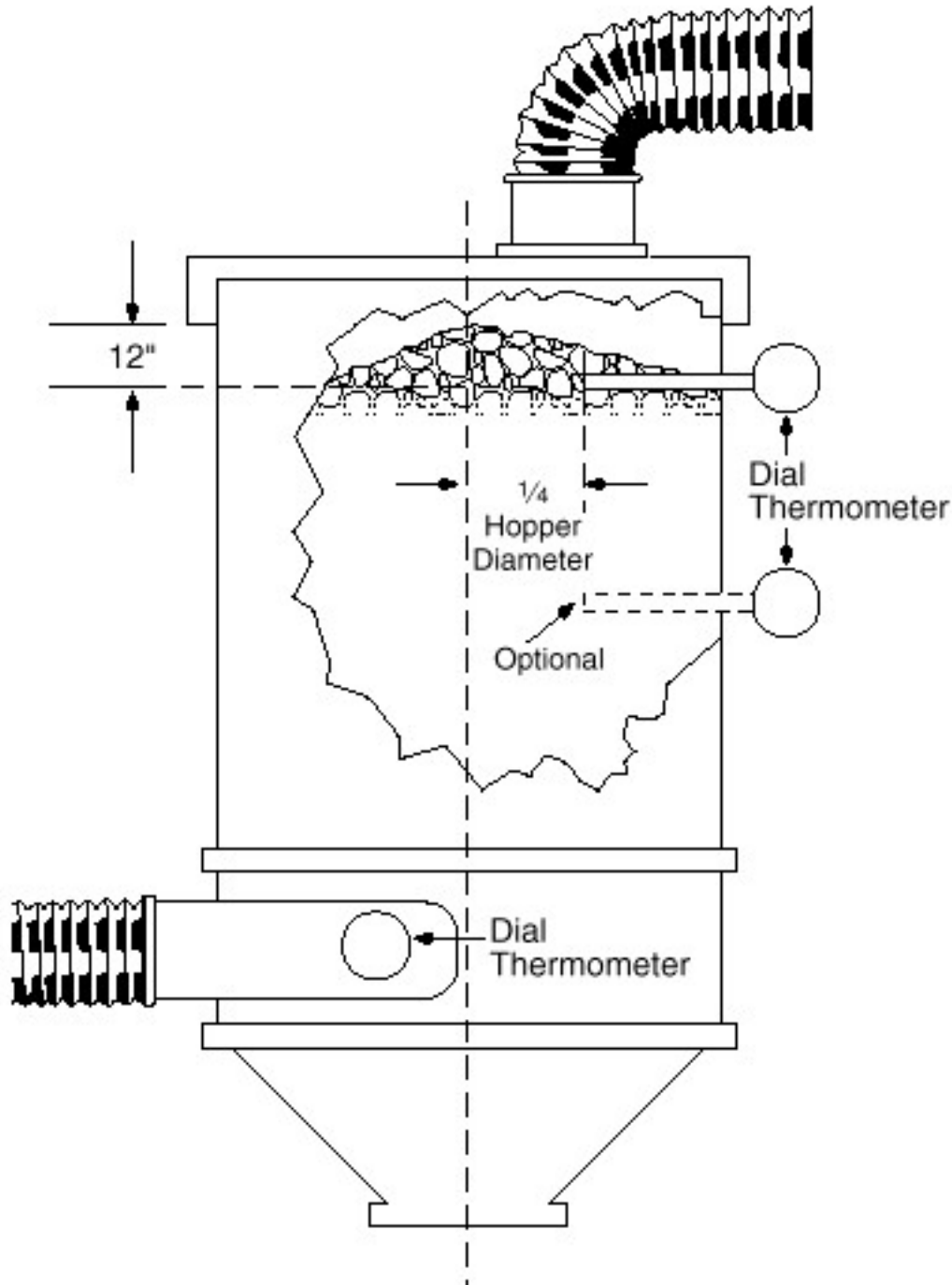
Figure 3-13. Closed Loop Desiccant Dryer.
