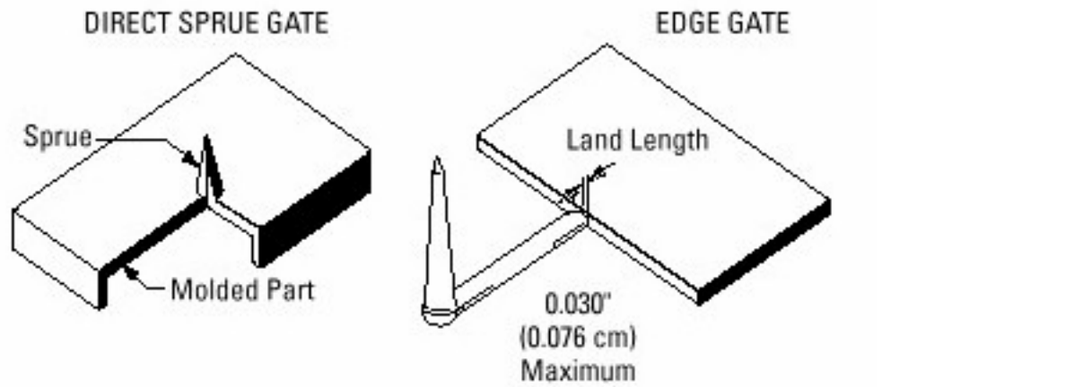
Figure 3-2. Sprue Gating.
