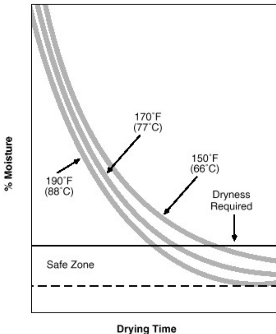
Figure 3-12. Drying Variables
