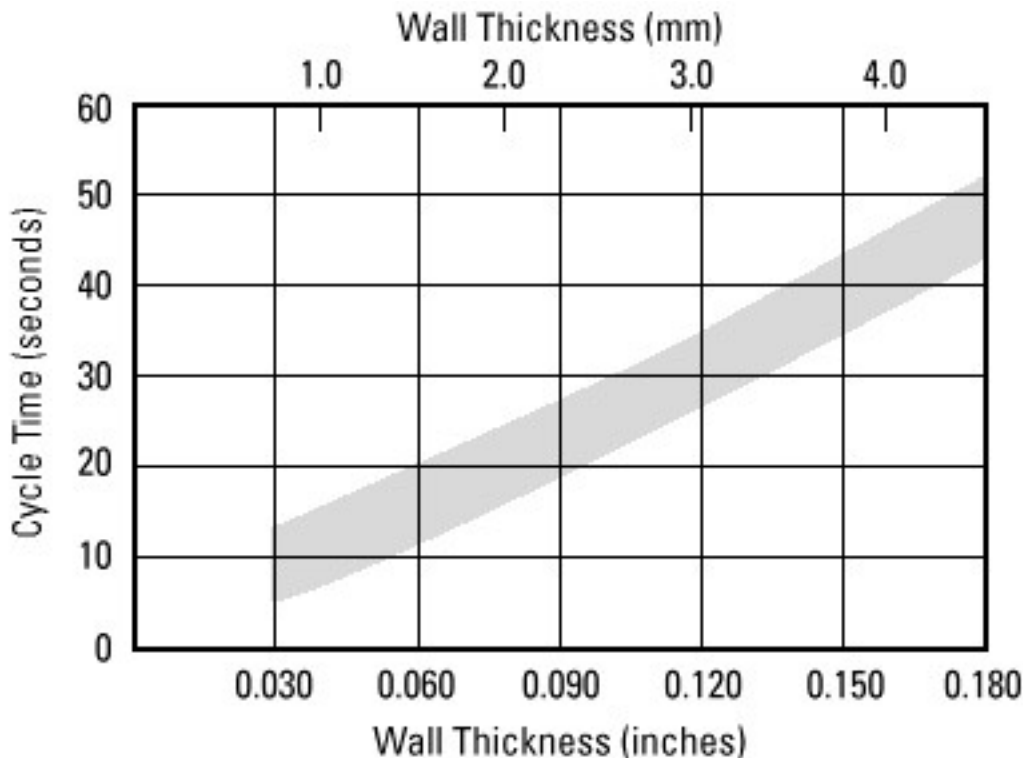
Figure 3-14. Typical Cycle Time Vs. Wall Thickness for CYCOLAC Resins
