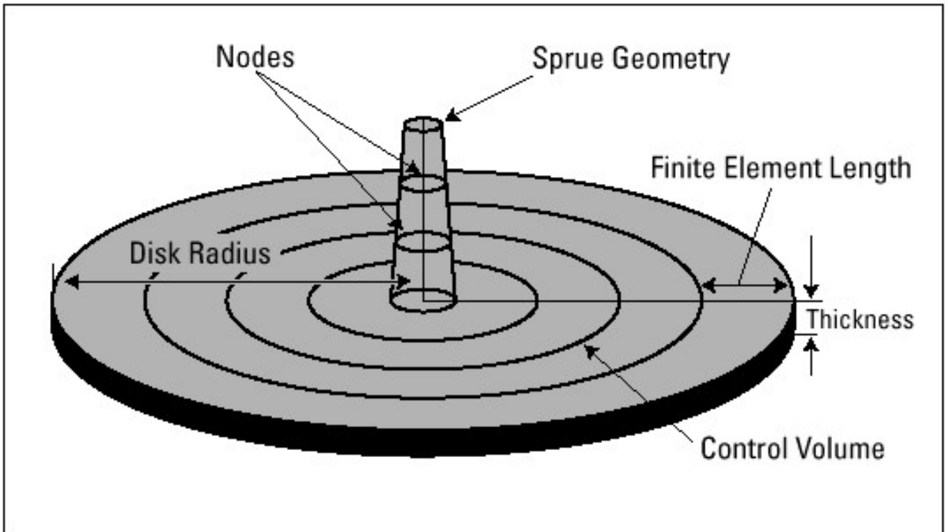
Figure 3-15. Diskflow Model
