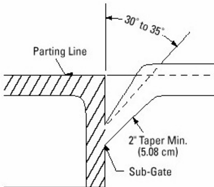
Figure 3-5. Tunnel Gate
